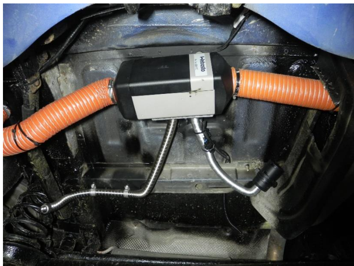
agregat Air Top 2000 STC
